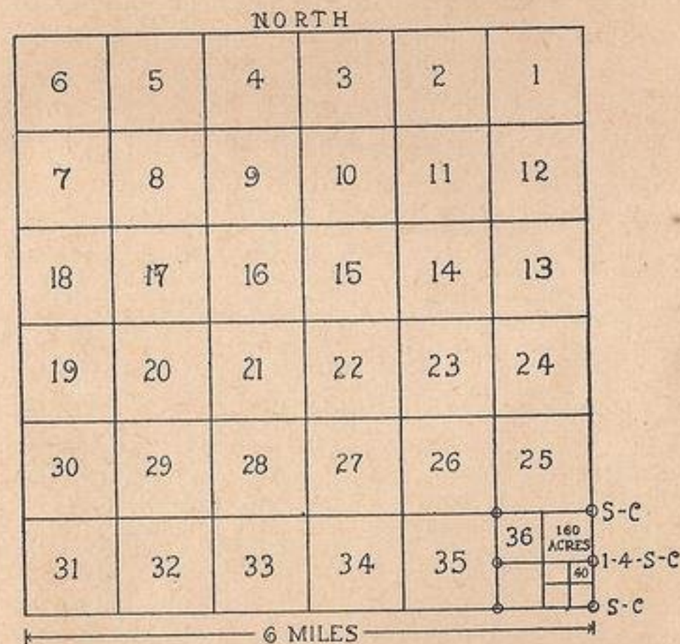
Township Diagram.
